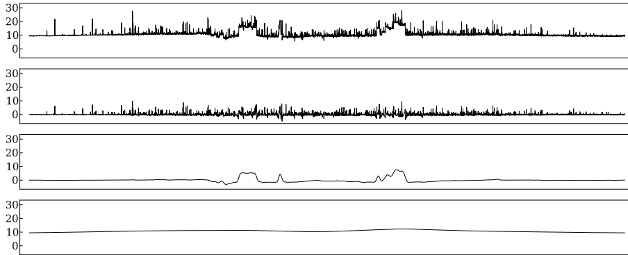
Fig. 6: Signal and top ranked scale decomposition for the InfraWatch data.
