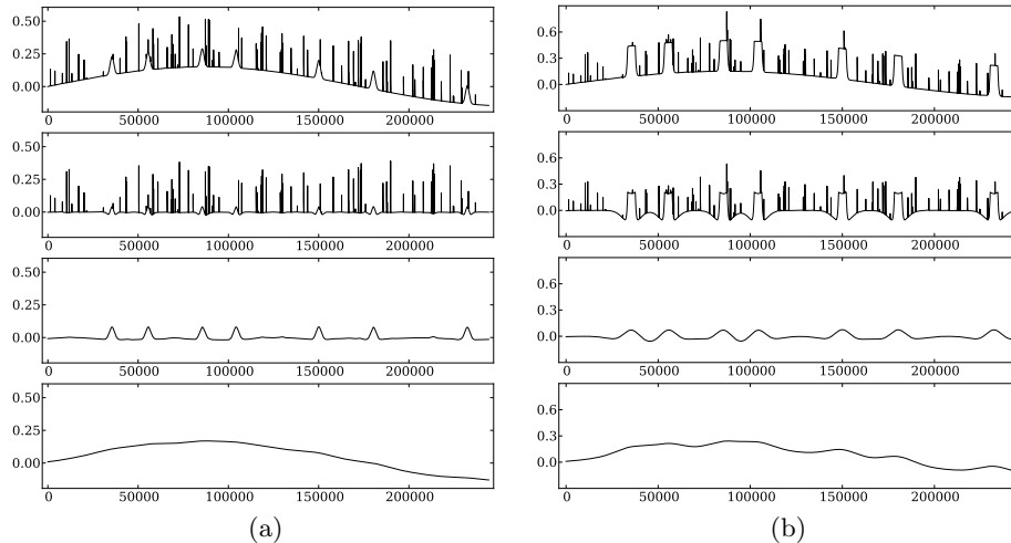
Fig. 5: Signals and top-ranked decompositions for the two artificial datasets.
